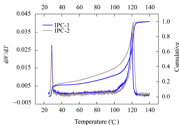
Fig. 1 TREF curves of the two impact propylene copolymers
